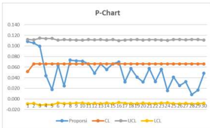
Gambar 2. Peta Kendali P ( P - Chart )
